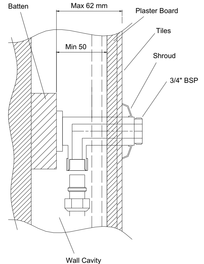
WALL PLATE
