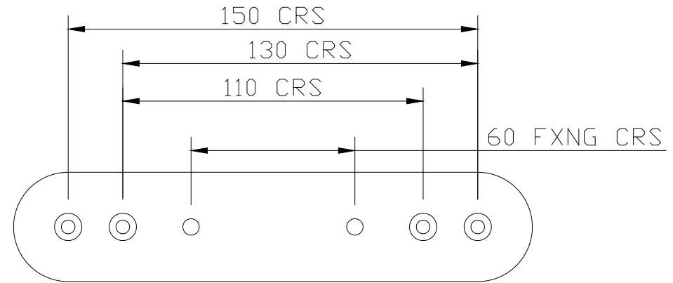
WALL PLATE
