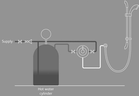
Typical UHW system installation
