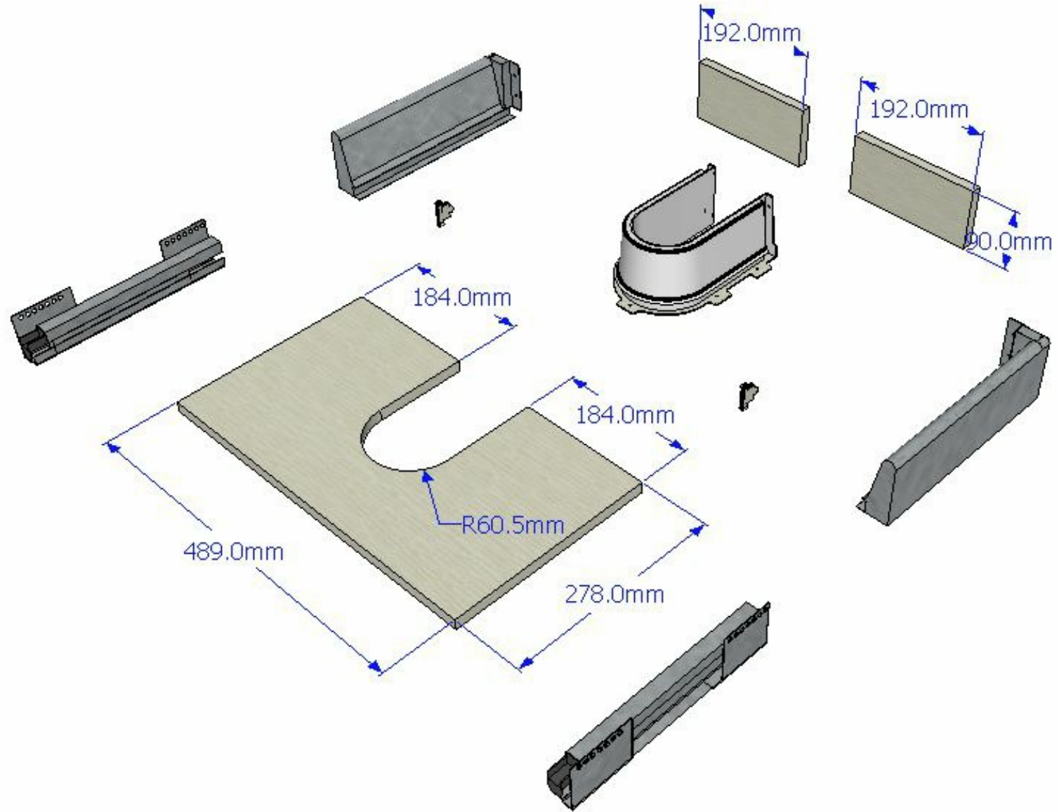
Top Drawer - Exploded View
