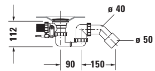
Siphon for whirltub # 760137
