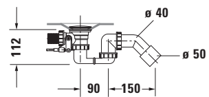
Siphon for whirltub # 760100
