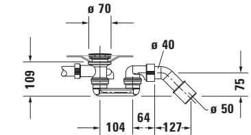
Siphon for bathtub # 700097
