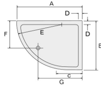
Offset LH Tray
