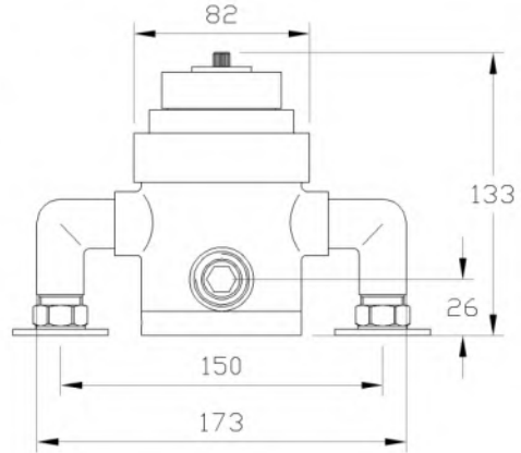
EXPOSED VALVE
