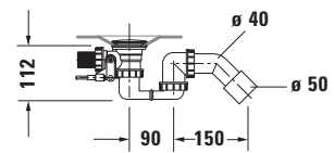
Siphon for whirltub # 760138
