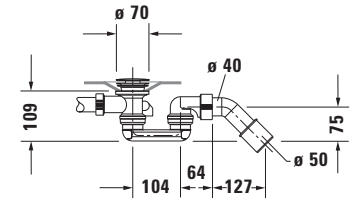
Siphon for bathtub # 700098
