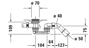
Siphon for bathtub # 700099
