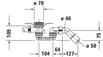
Siphon for bathtub # 700096
