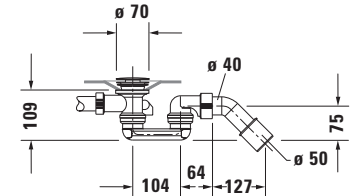
Siphon for bathtub # 700137
