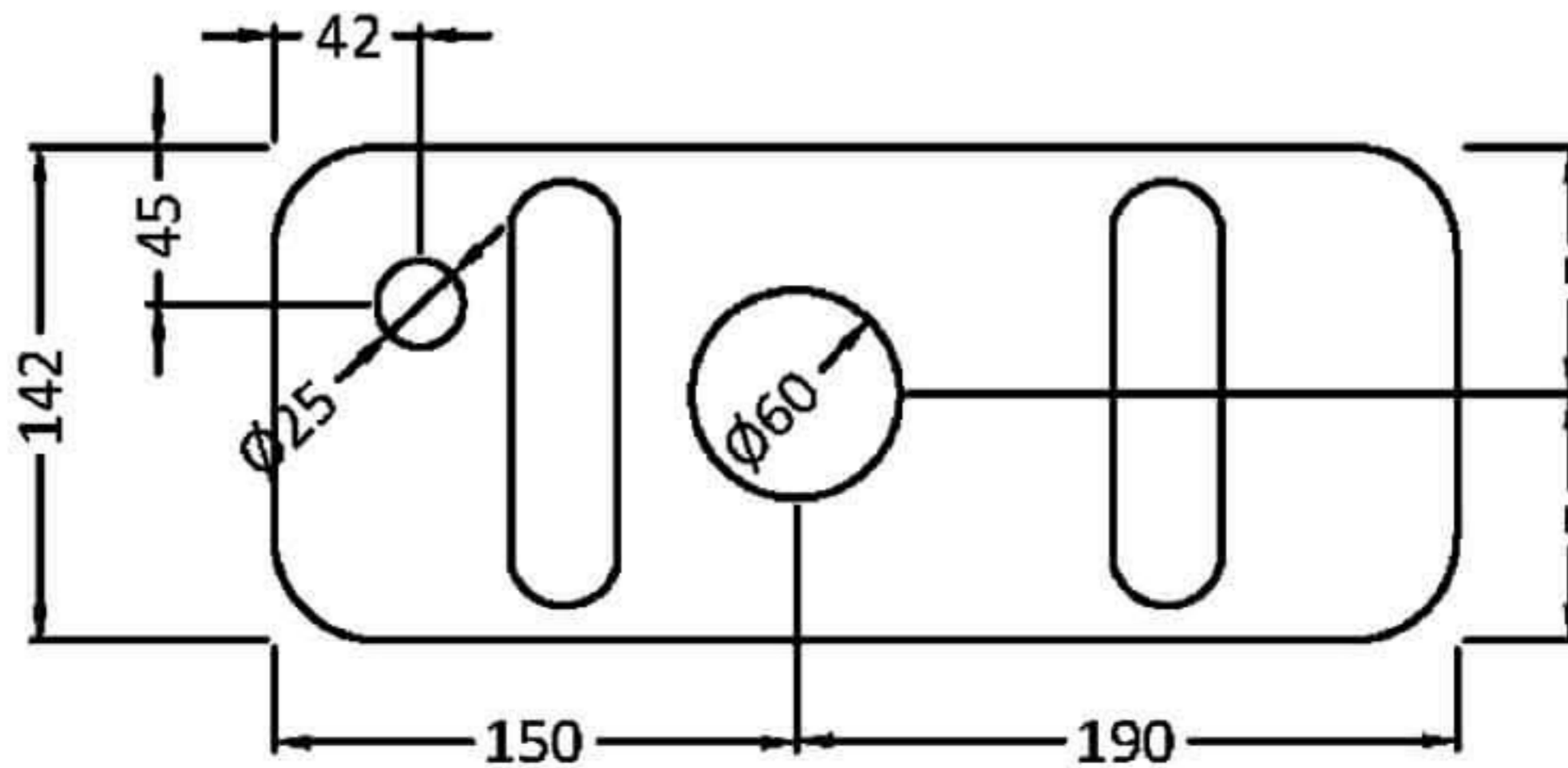
UNDERSIDE
