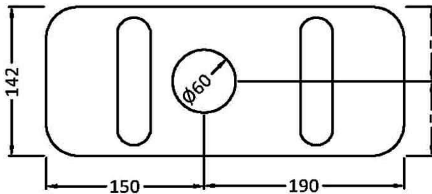
UNDERSIDE
