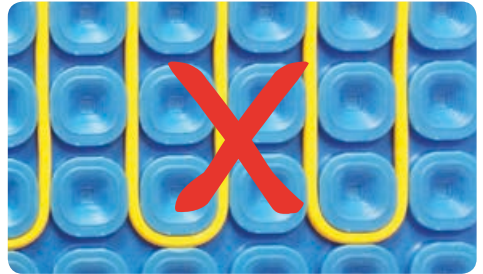
Incorrect heating cable spacing
