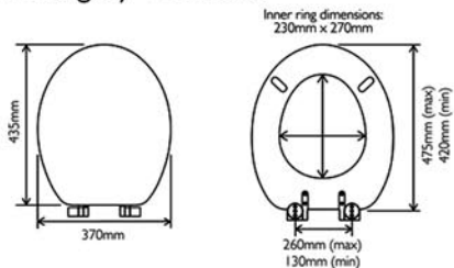
General seat dimensions
