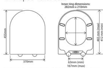
General seat dimensions
