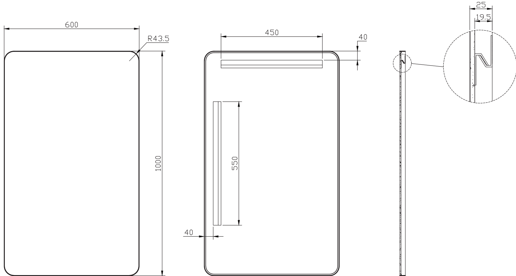
Front View
