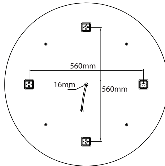
Back View
