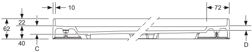
Side Profile of Uprstand Tray
