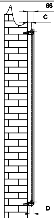
Side View
