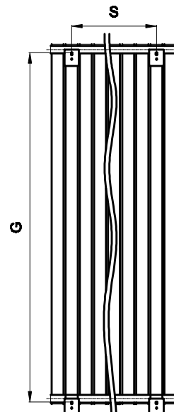
Back View
