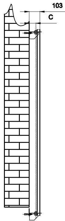
Side View
