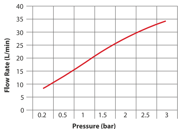
Flow Rates for 15mm Mixing Valves
